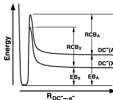
FIG. 2. Schematic potential energy curves explaining the observed photoelectron spectra of \text{DC}^{2-} . X and A represent the ground and excited states of the \text{DC}^{-} singly charged radical anion, accessed from the detachment of \text{DC}^{2-} . \text{EB}_X , \text{EB}_A , \text{RCB}_X , and \text{RCB}_A are the adiabatic binding energies and the repulsive Coulomb barriers for the X and A states, respectively. Note that \text{RCB}_X and \text{RCB}_A are assumed to have similar magnitudes for \text{DC}^{2-} (see text).
