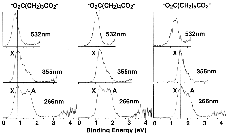
Fig. 1. Photoelectron spectra of DC^{2-} anions ( n = 3-5 ) at 266, 355, and 532 nm. Note the shift to lower binding energies of the 532 nm spectra relative to that of the 266 and 355 nm spectra. The vertical lines are drawn to guide the eyes.
