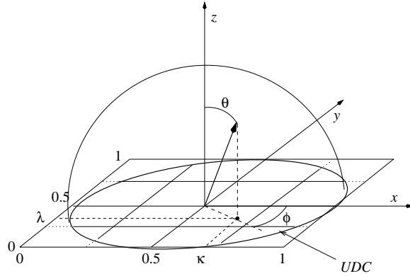
Figure 5.1: Nusselt Coordinates
