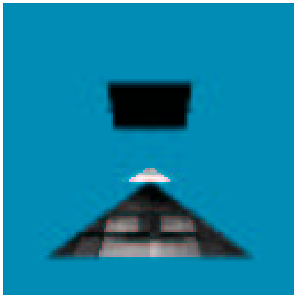
Figure 7.12: Lucifer Example
