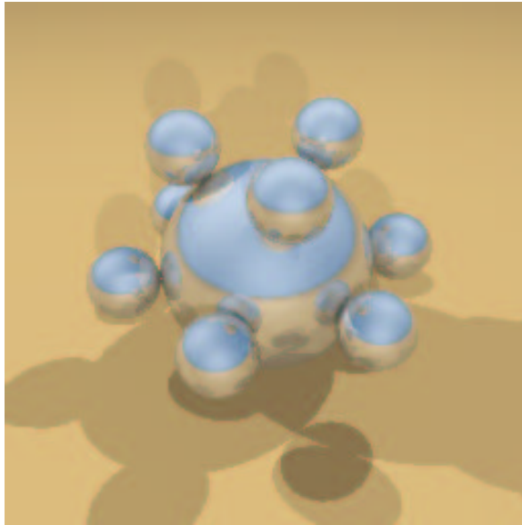
Figure 3.4: “Balls” Model
